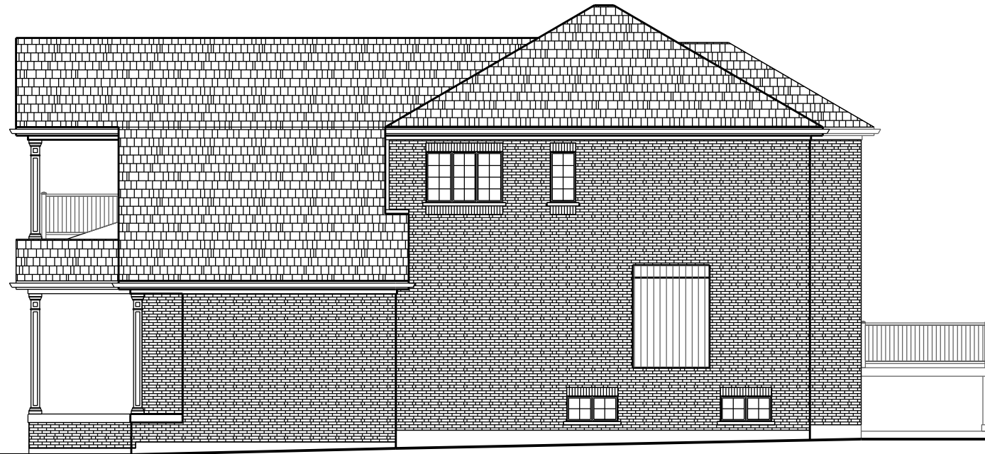
Right Side ( West ) Elevation
