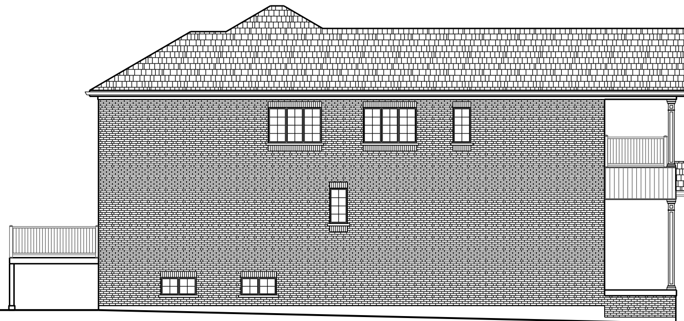
Left Side ( East ) Elevation
